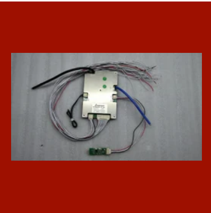
19S 60V 40 Amp Smart BMS
